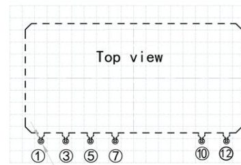
PCB layout vertical view Grid 2.54x2.54[0.10x0.10]
