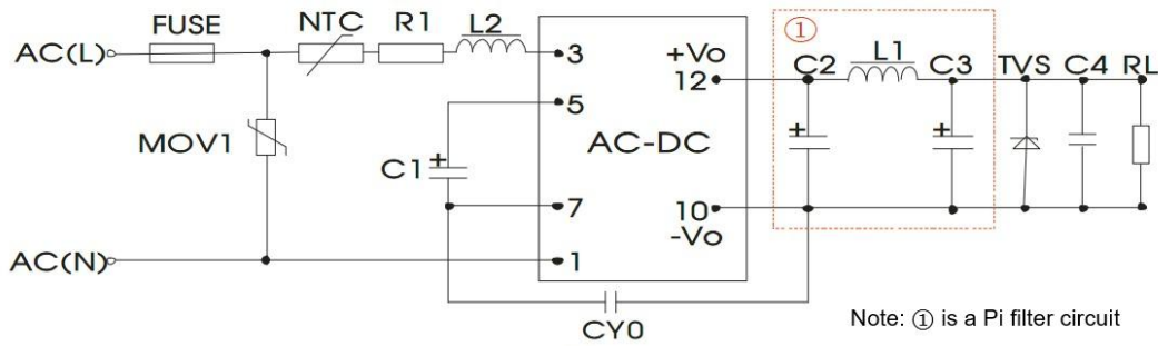
Figure - Circuit 1
