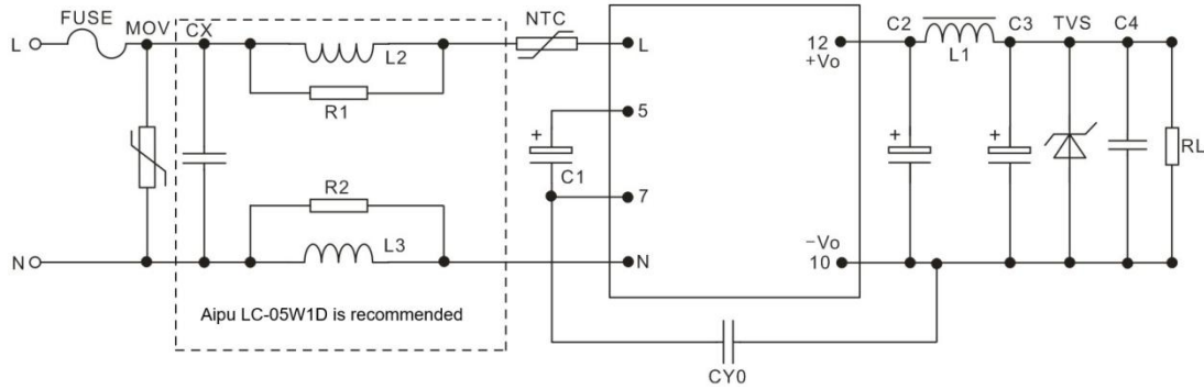
Figure – Circuit 2/2
